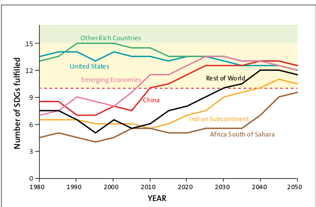
Figure 2.1.3 SDG success score per region 1980–2050 in scenario Same .
